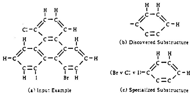
Figure 1. SUBDUE Example
