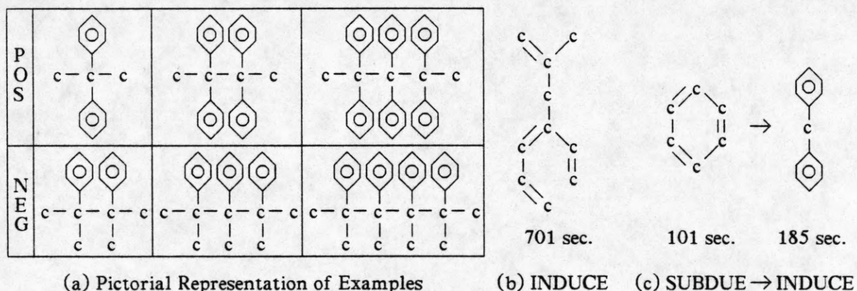
Figure 4. SUBDUE/INDUCE Example
