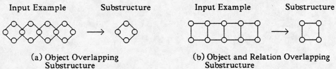
Figure 2. Overlapping Substructures
