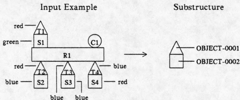
Figure 1. Example Substructure
