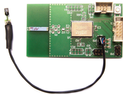
Figure 3. The Pixie node is a flexible prototyping platform which is equipped with extension headers for external peripherals. In this picture, a Sensirion SHT75 temperature/humidity sensor is attached to the node.
