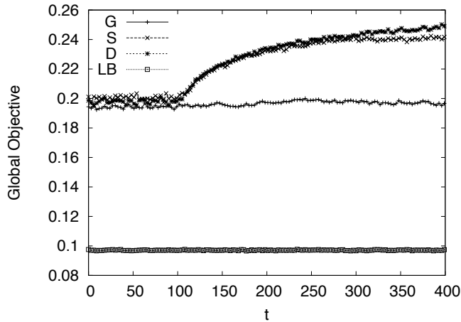
Figure 3: Simulations results for 50 servers with 4 agents each with parameter values ( r=0.8, M=8 ). For this hard problem, load balancing performs very poorly, and agents using tailored objectives S and D perform significantly better than agents using G .
