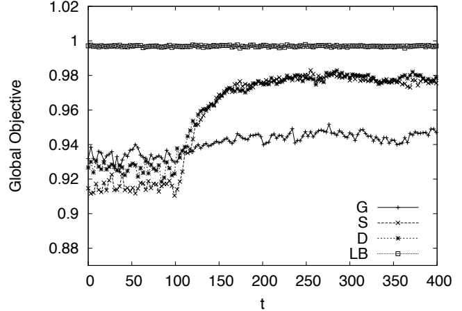
Figure 1: Simulations results for 50 servers with 4 agents each with parameter values: ( K=2, r=0.2, M=2 ). Each t represents a “run” of 400 \tau time steps with each agent having a fixed probability vector \vec{p} during the run. At the end of each run, objectives are calculated, the queues cleared, and the agents reset/modify their \vec{p} based on their learning algorithms. Results are averages over 50 different systems configurations, and error bars (differences in the mean) are less than .01 in all figures.
