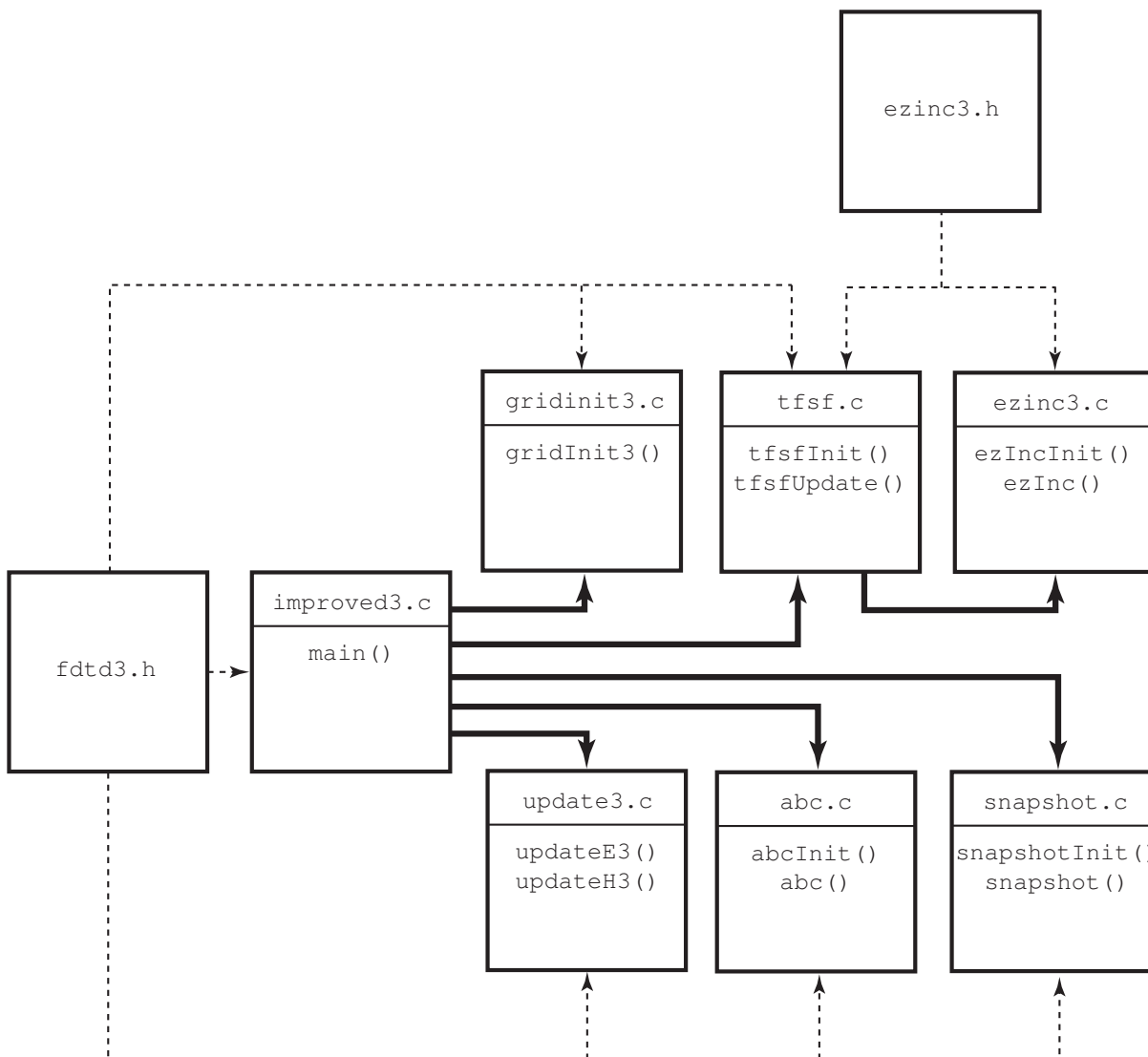
Figure 4.3: The files associated with the third improvement of the FDTD code. The header file ftd3.h is explicitly included in the source files to which it is joined by a dashed line. (Wherever ezinc3.h appears it also ensures ftd3.h is included.) The file improved3.c contains the main() function but the initialization of the grid, the application of the absorbing boundary condition, the calculation of the source function, the updating of the fields, and the taking of the snapshots is no longer done in main() . Instead, other functions are called to accomplish these tasks.
