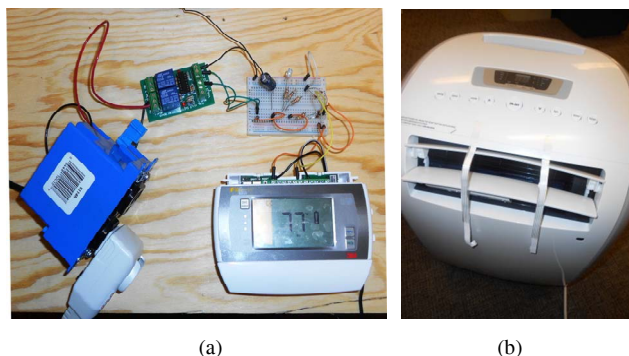
Fig. 4. The HEM system setup in our laboratory: (a) the smart thermostat with its control circuit, (b) the portable AC unit controlled by the thermostat.
