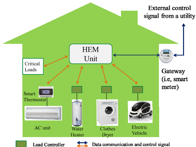
Fig. 1. Overall HEM system architecture with smart thermostat.
