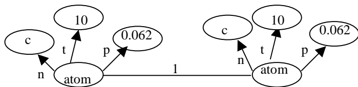
Figure 2: Substructure S_3 .
