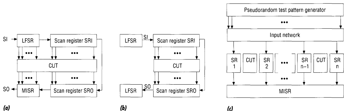
(a) (b) (c) Figure 2. Test-per-scan configurations.
