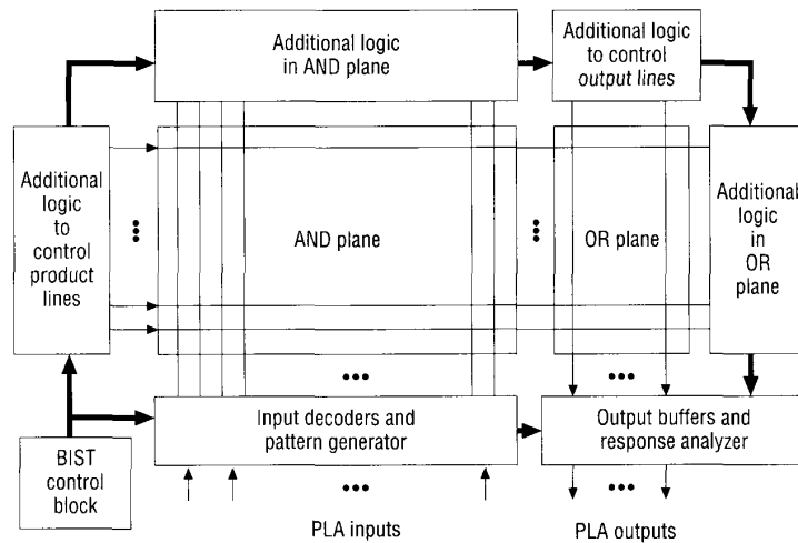
Figure 5. A generic BIST architecture of PLAs.
