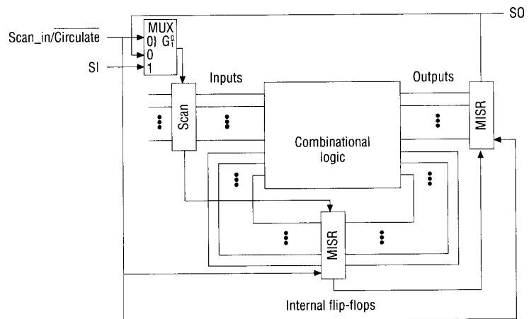
Figure 4. General full-circular BIST configuration.
