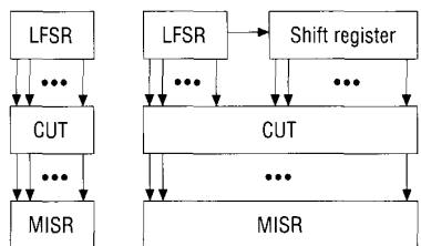
(a) (b) Figure 1. Test-per-clock configurations.
