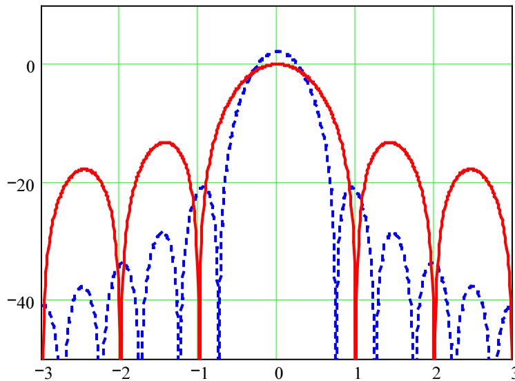
Figure 22.3: BPSK spectrum (solid red curve) compared to MSK spectrum (dashed blue curve). Both curves have unit energy (on linear scale). Horizontal axis is normalized frequency fT_b , relative to the carrier, vertical axis is amplitude in dB.
