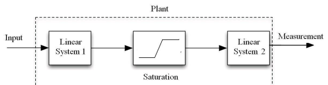
Fig. 2. Sandwich system with saturation nonlinearity and partial-state measurement from second subsystem only
