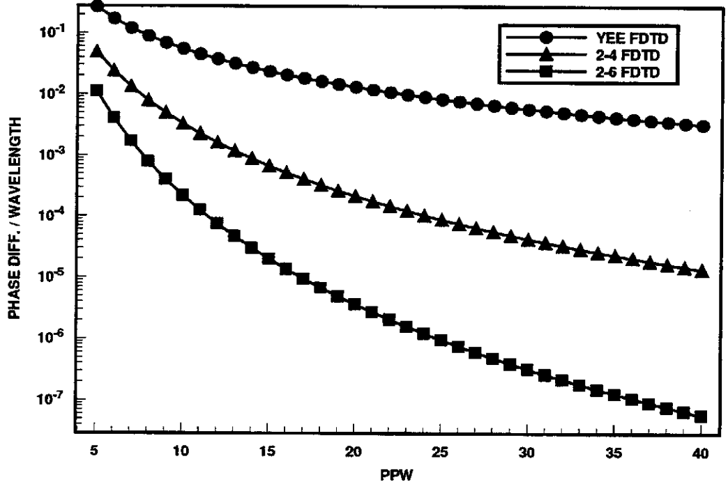
Figure 3: Phase difference between plane wave traveling at 0° and 45° with respect to the grid lines per wavelength curves for the YA, 2-4 and 2-6 methods versus points per wavelength (PPW) discretization.
