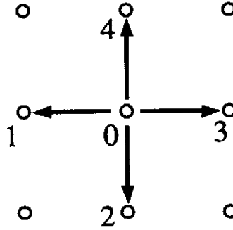
Figure 1: Nodes in the computational mesh.
