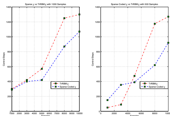
Fig. 5. Performance comparison of transferring from IP to CP using FTrRBM or Sparse Coded inter-task mappings (i.e., Bou Ammar et.al [3]). The left graph shows the results of transfer when using 1000 target samples to learn the intertask mapping, while the right presents the results when using 500 samples to learn such a mapping.
