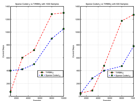
Fig. 6. Performance comparison of transferring from MC to CP using FTrRBM or Sparse Coded inter-task mappings (i.e., Bou Ammar et al. [3]). The left graph shows the results of transfer when using 1000 target samples to learn the intertask mapping, while the right presents the results when using 500 samples to learn such a mapping. It is clear that FTrRBM transfer outperforms that described in [3].
