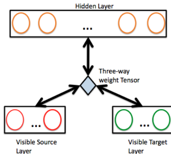
Fig. 1. The overall structure of the proposed full model. The three-way weight tensor is shown in the middle with its connections to each of the visible source layer, visible target layer, and the hidden layer shown in red, green, and orange respectively.
